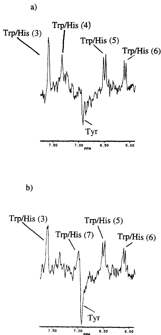
Fig. 3. Spectrum of mock-treated (a) and sialidase-treated SAP (b), which shows the strong decrease of Trp/His signal 4, the appearance of Trp/His signal 7 and the increase in intensity of the Tyr signal.
